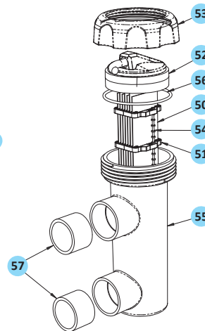
ELECTRODE CELL PARTS
